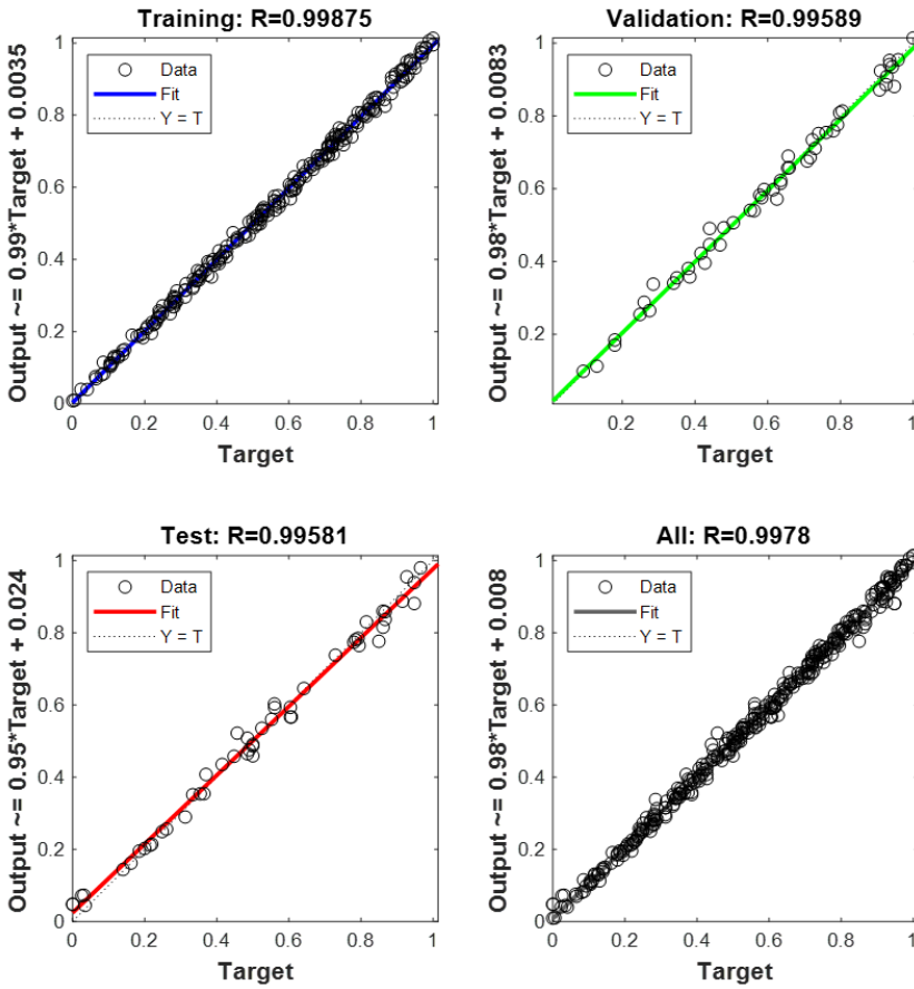
Fig. 10. Correlation analysis diagram of BP neural network structure.
