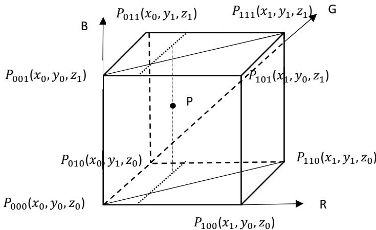
Fig. 4. Cube structure diagram for 3D interpolation.
